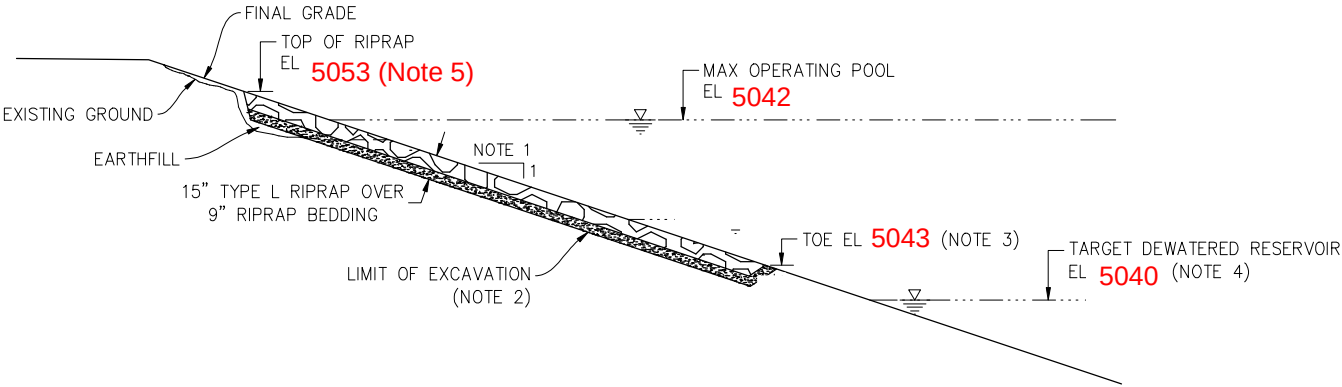
TYPICAL SECTION
