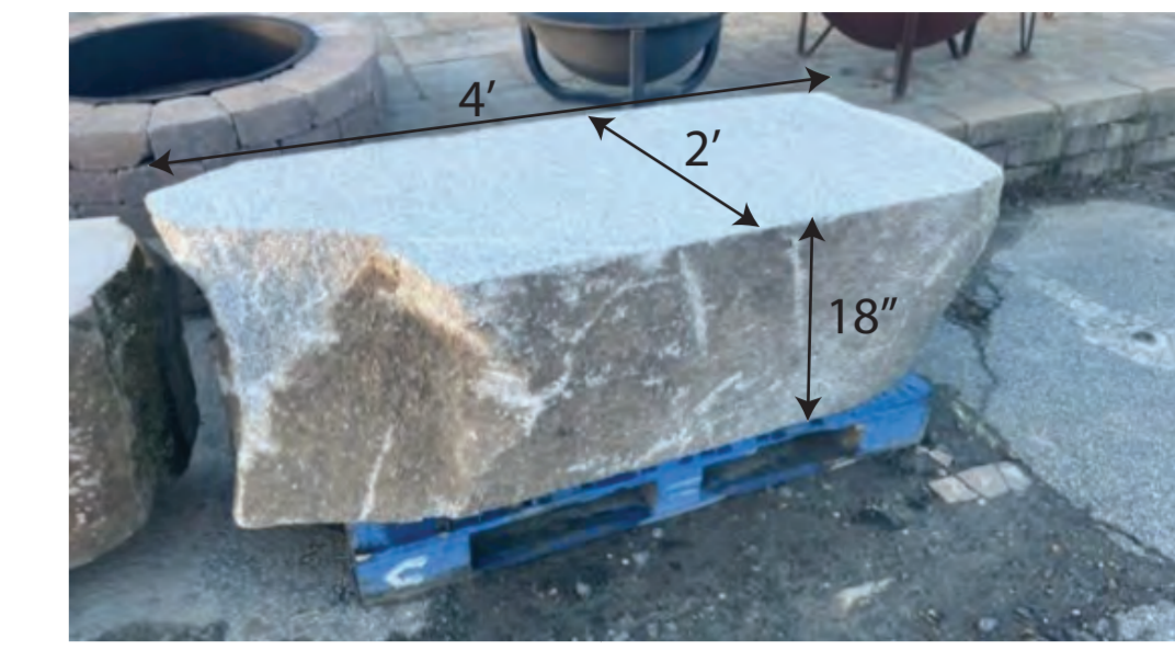
2 SAWN TOP SEAT BOULDER NOT TO SCALE
