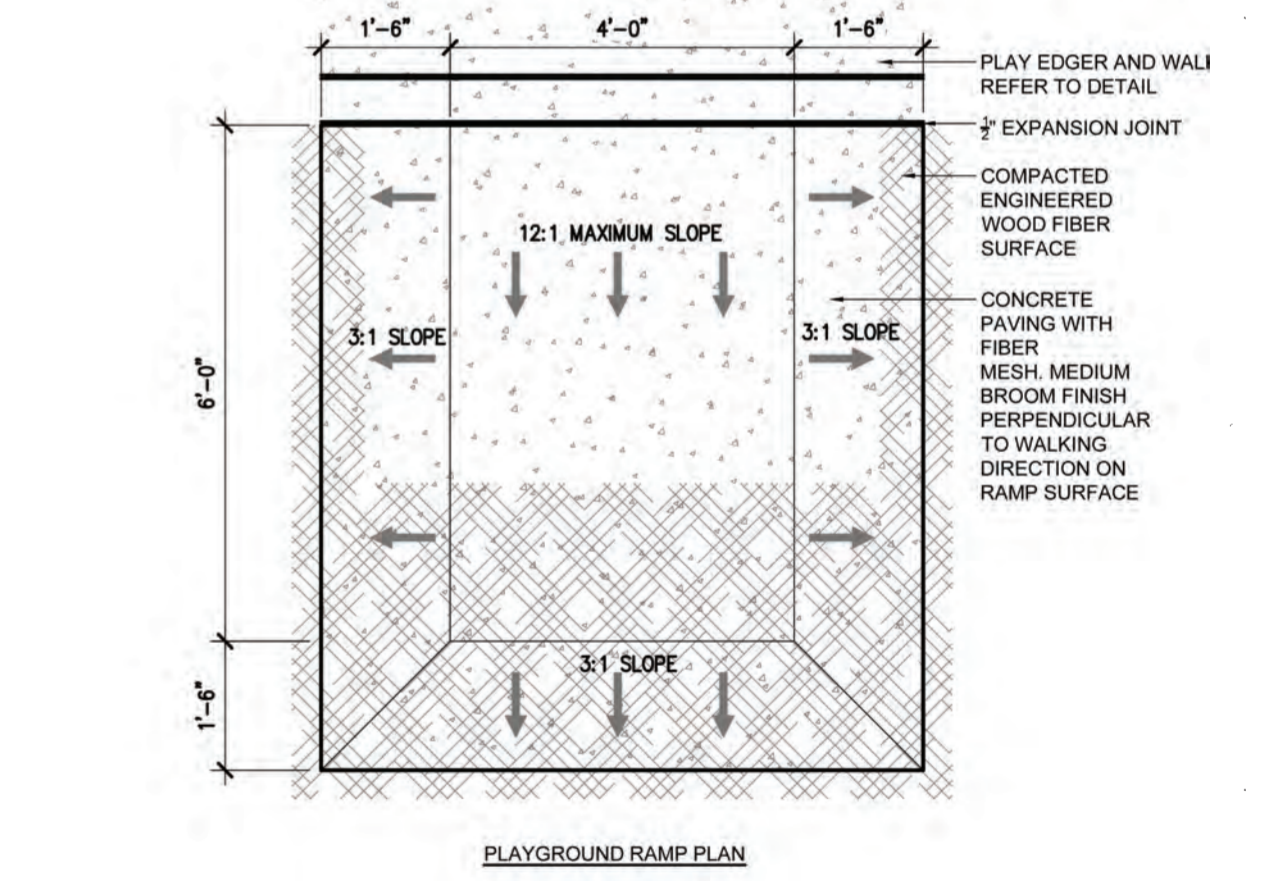
4 ADA PLAYGROUND RAMP SCALE: 3/4" = 1'-0"
